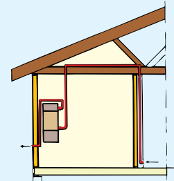
Fig. 4 Piping in the attic
